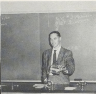
Mr. Bell shows chemical reaction with an experiment in chemistry.
